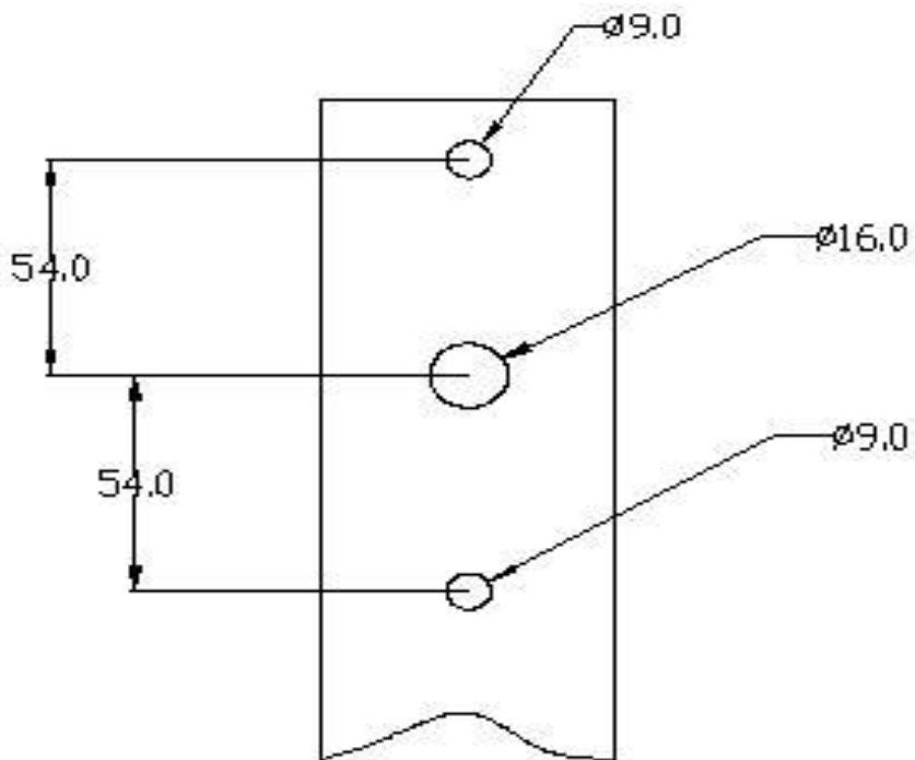
Fixed lamp square tube hole location
