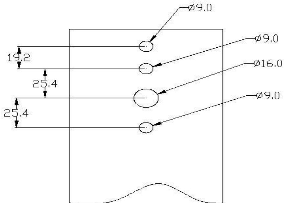
Fixed lamp tube hole position
